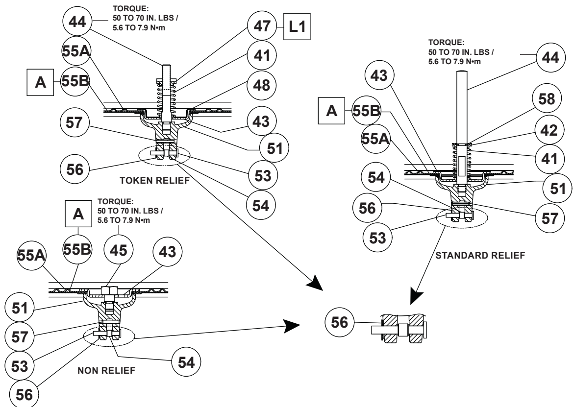
Figure 8. CS400 Series Regulator Assemblies (continued)
