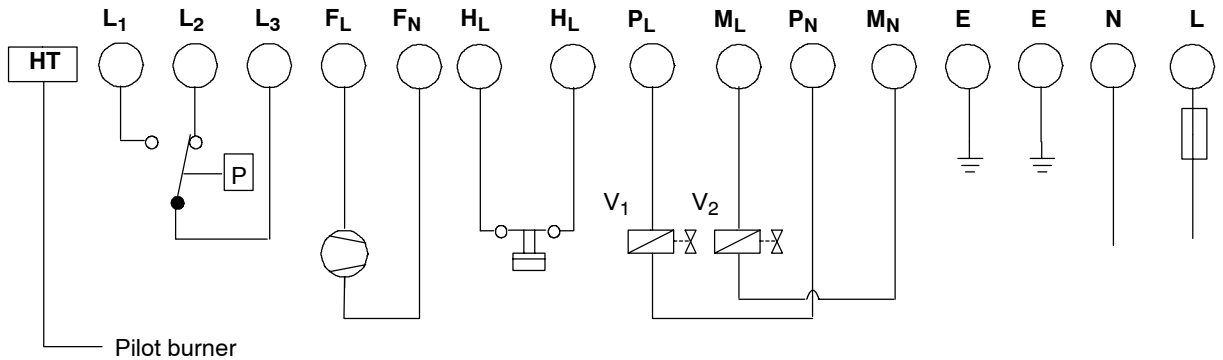
Fig. 2. Connection diagram S458 ignition control
